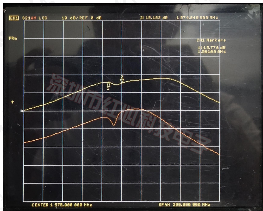
(Gain)增益图
