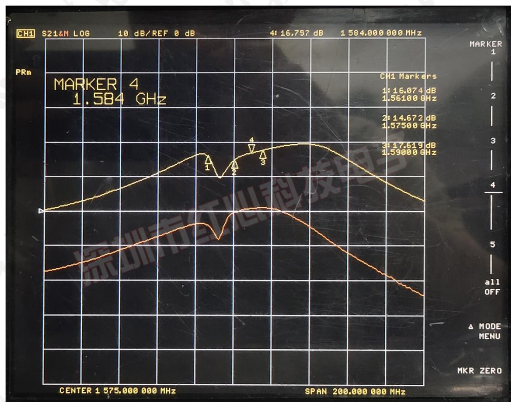
(Gain)增益图
