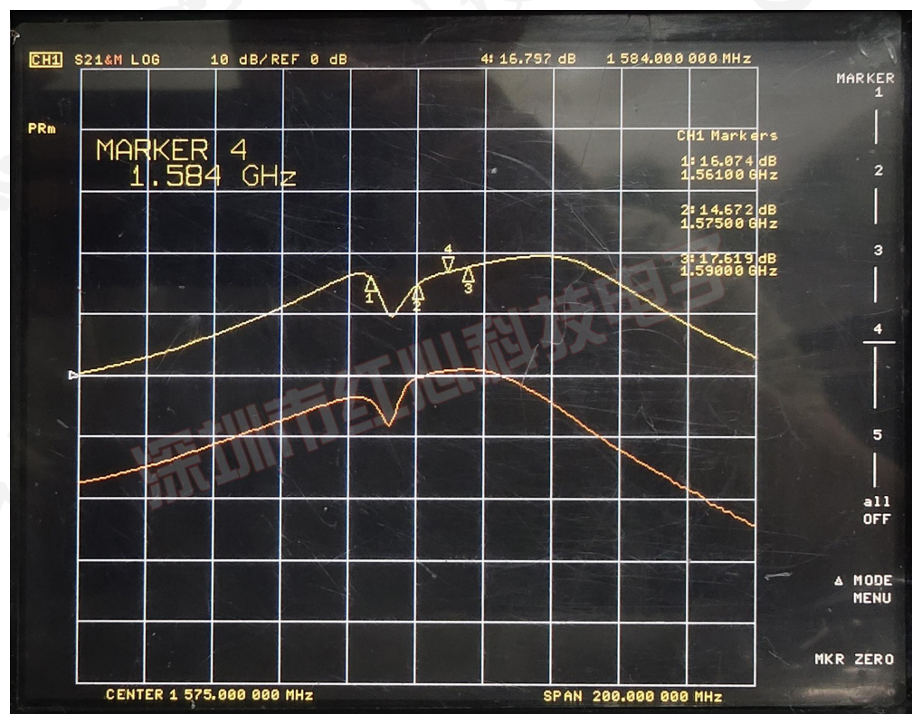
(Gain)增益图
