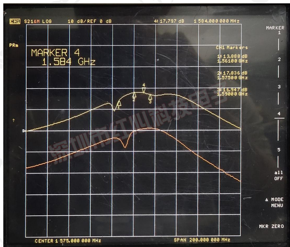
(Gain)增益图
