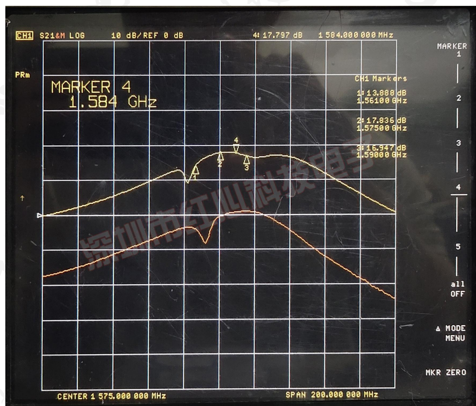
(Gain)增益图
