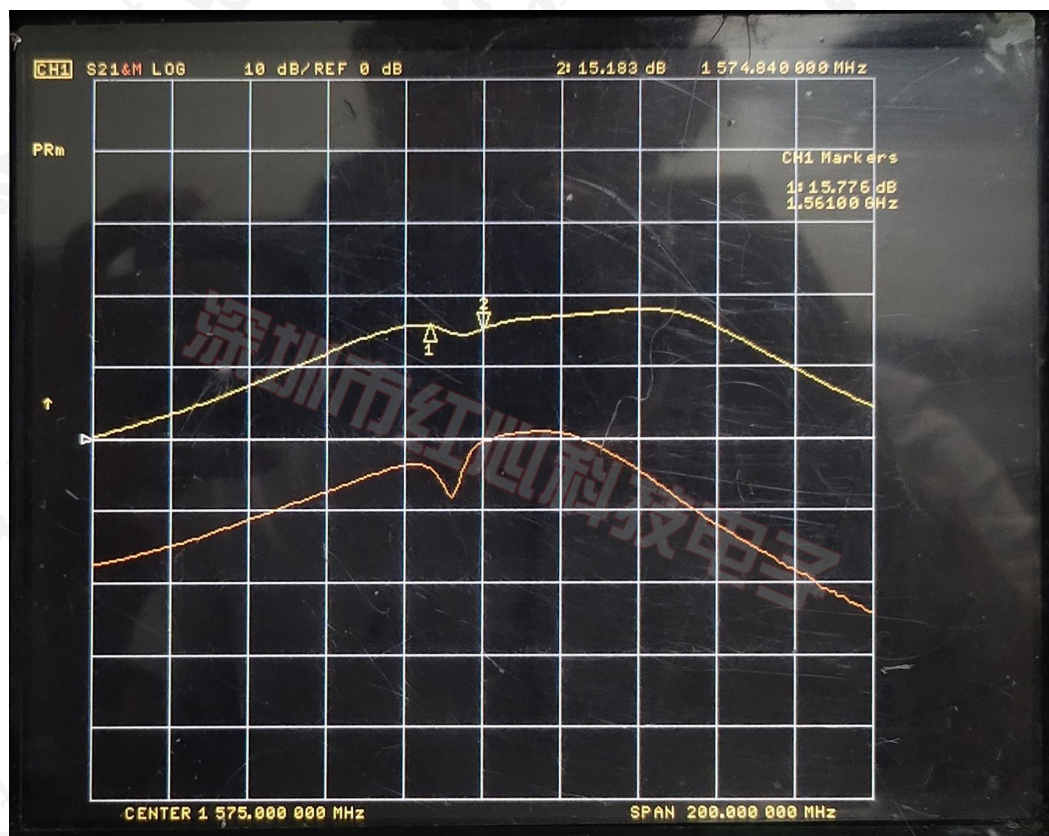
(Gain)增益图
