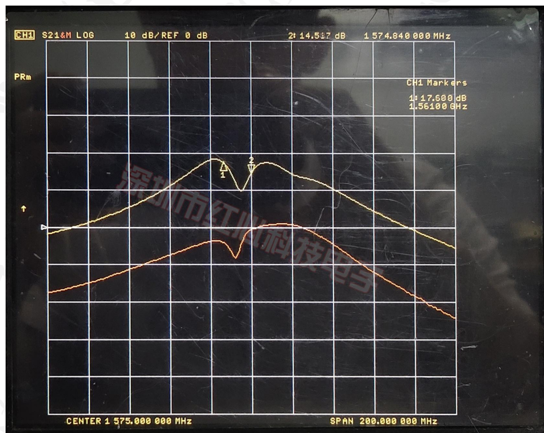
(Gain)增益图
