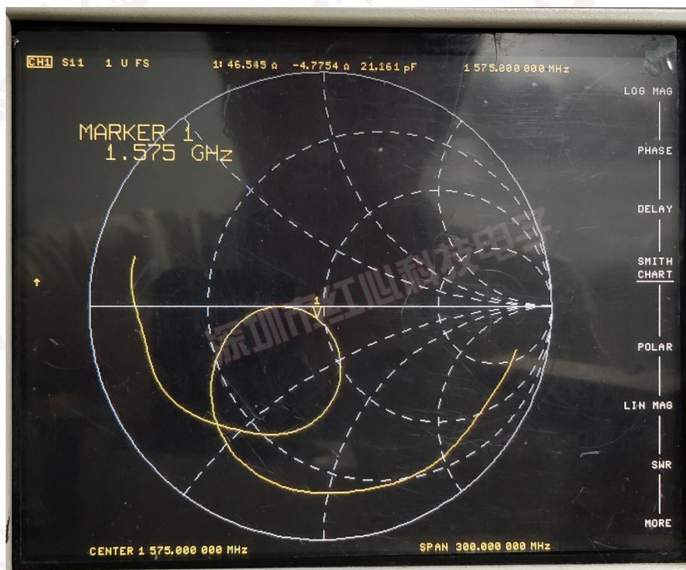
Smith Chart (史密斯圆图)
